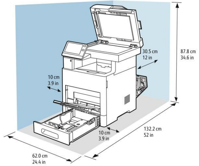
Xerox® VersaLink® B605/B615 Install Space:
