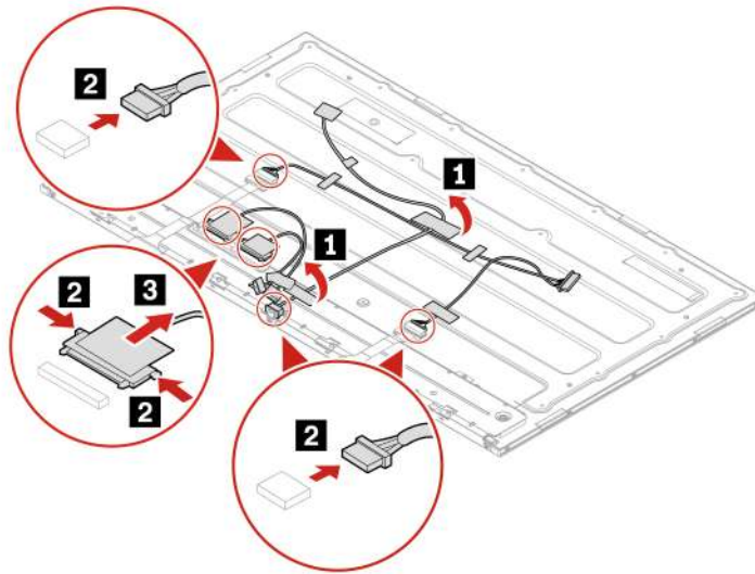
Figure 1. Remove the LCD power cable, the LVDS cables, and the focus sound screen cable from a focus sound screen
