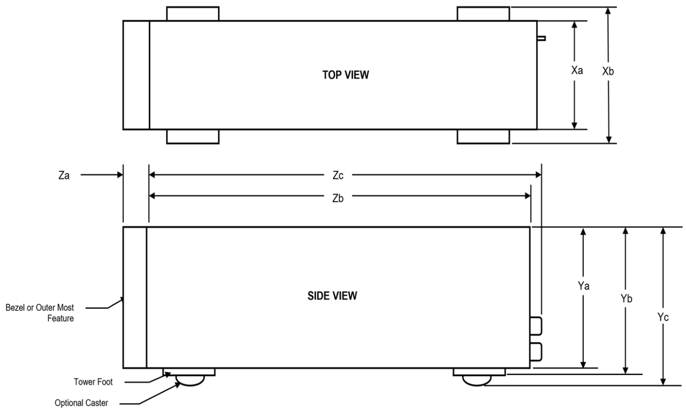
Figure 15. Chassis dimensions
