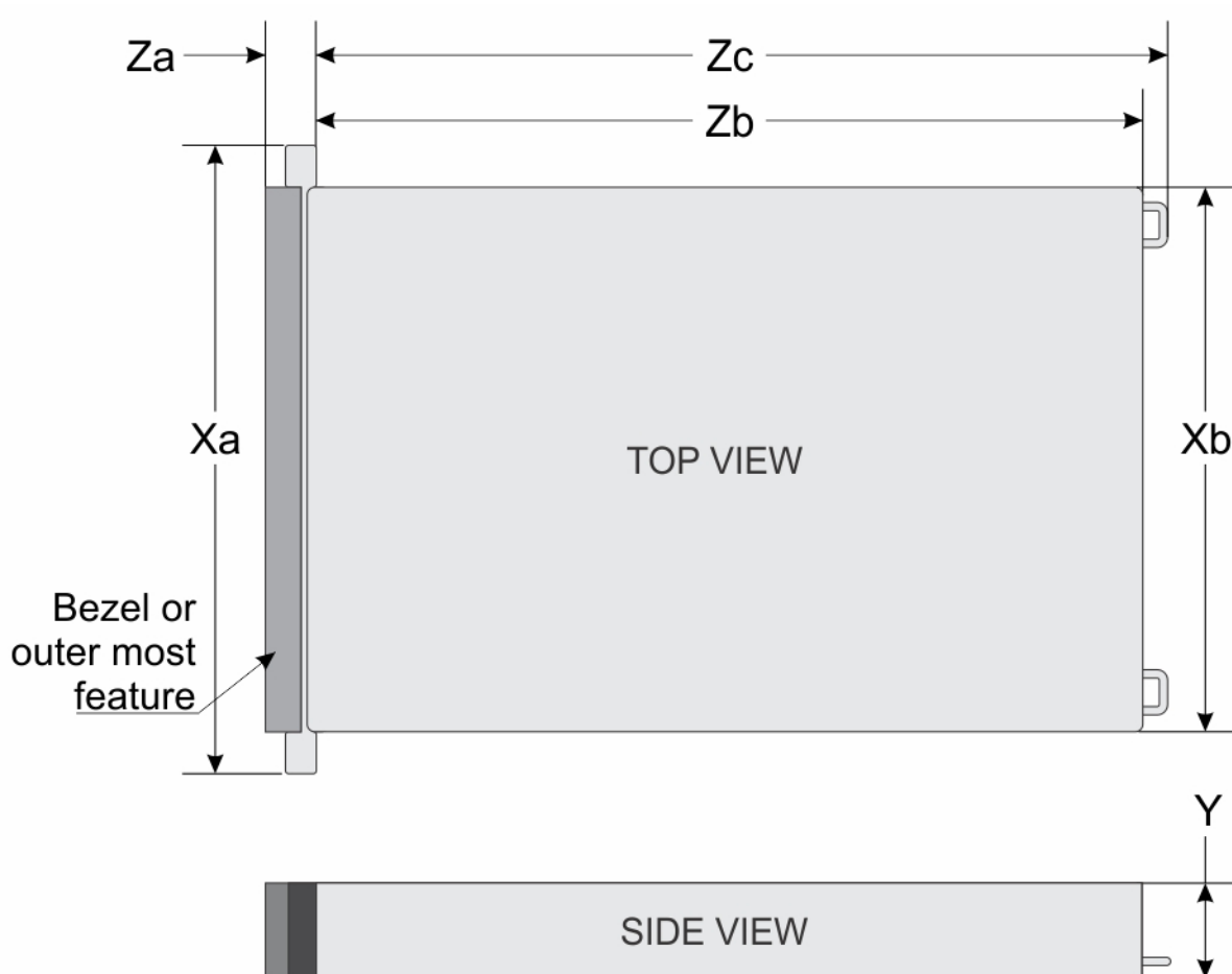
Figure 53. Chassis dimensions
