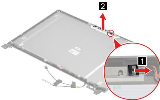
Figure 46. Disconnect the camera cable from the camera board and remove the camera
