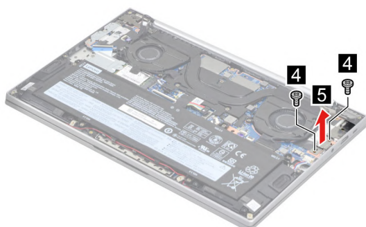
Figure 65. Remove two screws and remove the I/O bracket (left)
