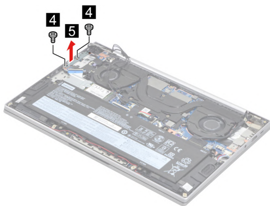
Figure 62. Remove two screws and remove the I/O bracket (right)
