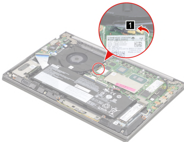
Figure 86. Peel off the mylar
