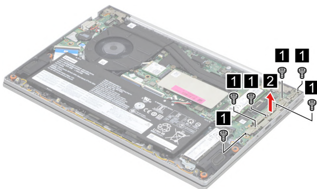
Figure 22. Remove six screws and then remove the I/O bracket (left)
