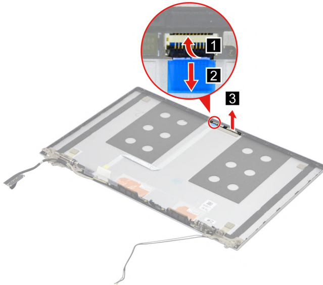
Figure 45. Disconnect the EDP cable from the camera board and remove the camera
