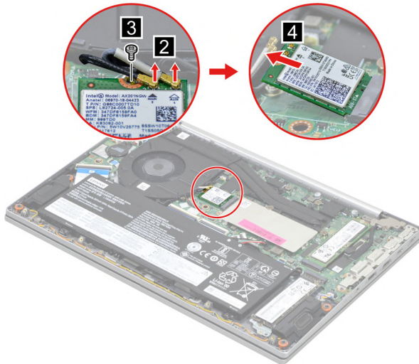
Figure 16. Remove one screw and remove the Wi-Fi card by pulling it away from the slot
