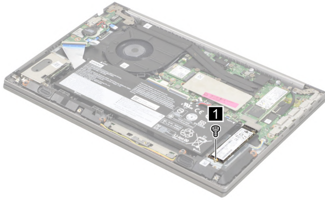
Figure 53. Remove one screw
