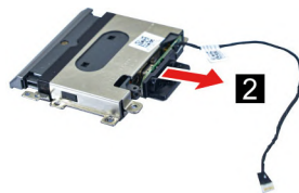
Figure 80. Remove the Bluetooth board module
