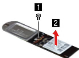
Figure 8. Remove one screw and separate the 2242 SSD from the SSD bracket
