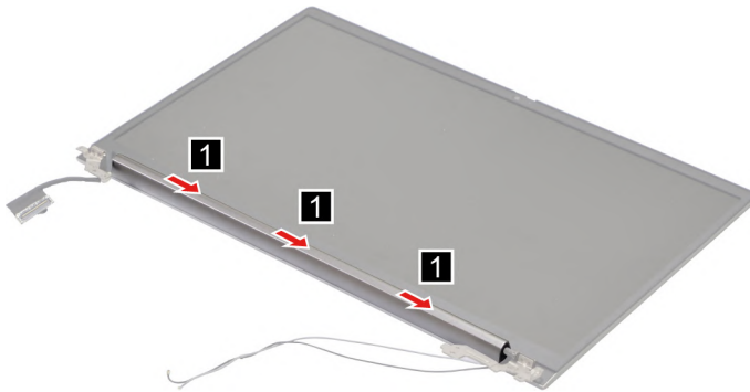
Figure 89. Remove the hinge cover
