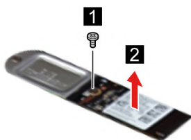
Figure 50. Remove one screw and separate the 2242 SSD from the SSD bracket
