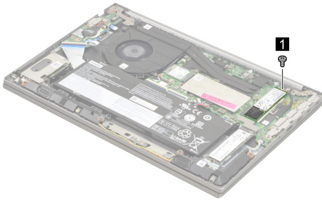
Figure 51. Remove one screw
