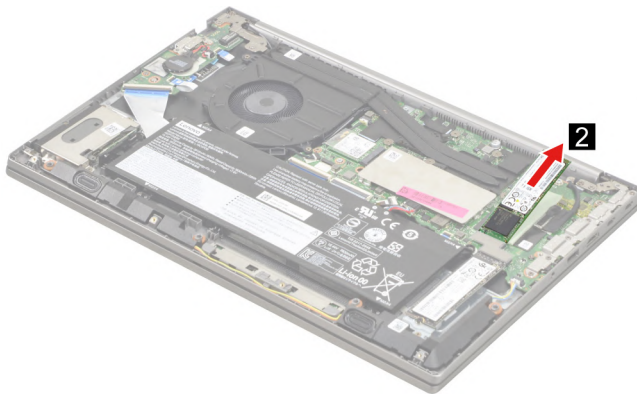
Figure 52. Remove the SSD by pulling it away from the slot
