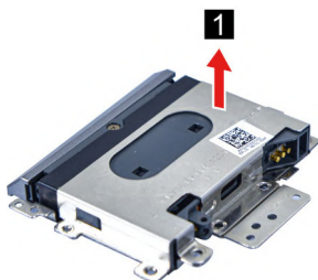
Figure 83. Open the buckles and separate the ear phone bracket from the ear phone tray module
