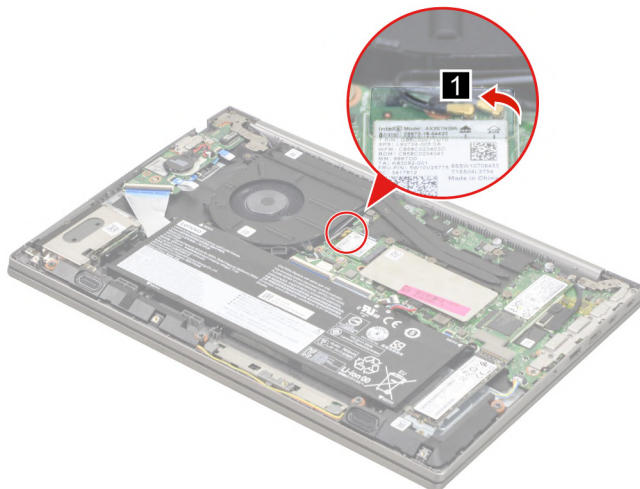
Figure 57. Peel off the mylar
