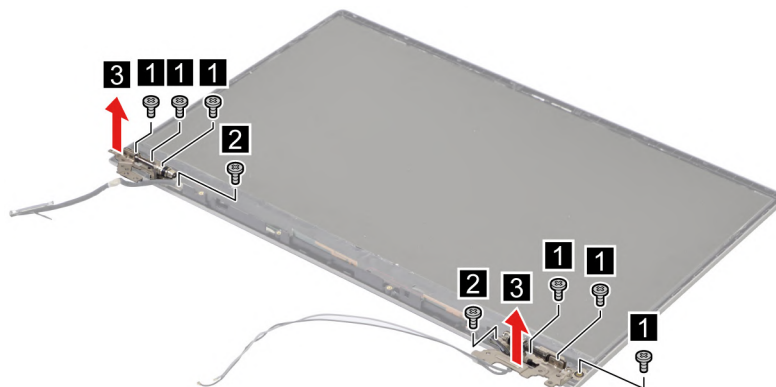
Figure 92. Remove eight screws and remove the hinges
