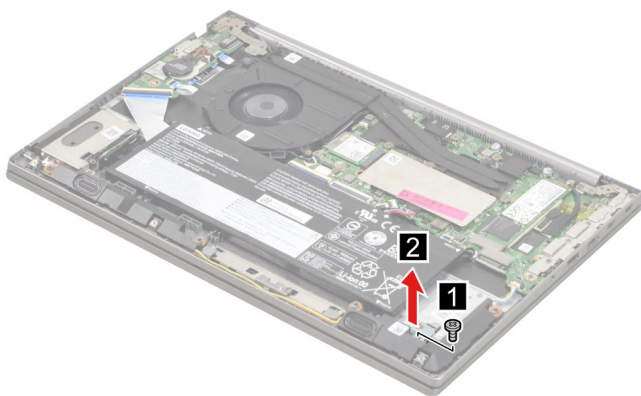
Figure 55. Remove one screw and remove the 2 nd SSD bracket
