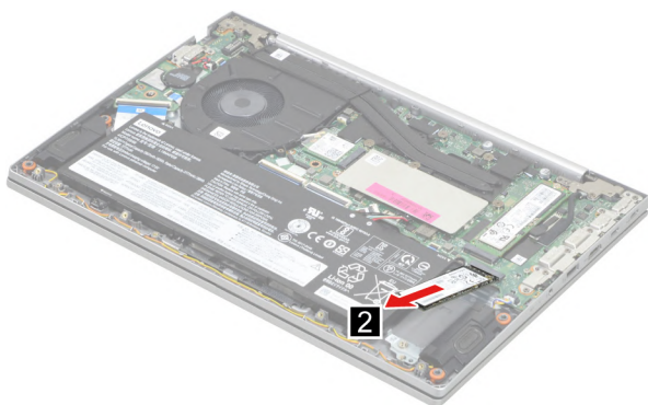
Figure 12. Remove the 2 nd SSD by pulling it away from the slot
