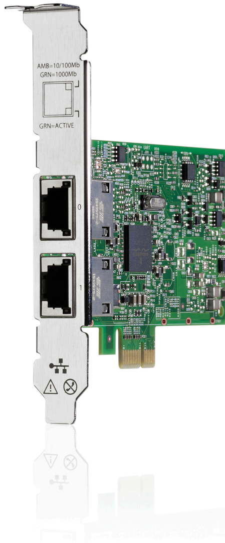
HPE Ethernet 1Gb 2-port 332T Adapter, with full-height bracket
