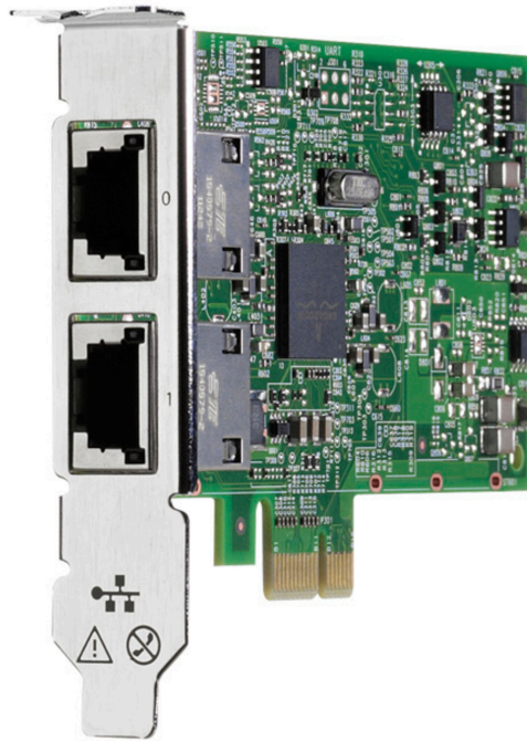
HPE Ethernet 1Gb 2-port 332T Adapter, with half-height bracket
