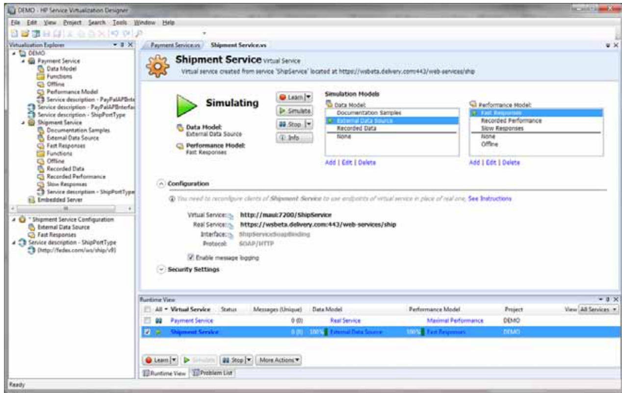
Figure 2. HP Service Virtualization Designer in simulation mode
