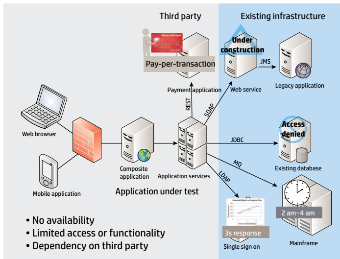
Figure 1. Composite application testing limitations
