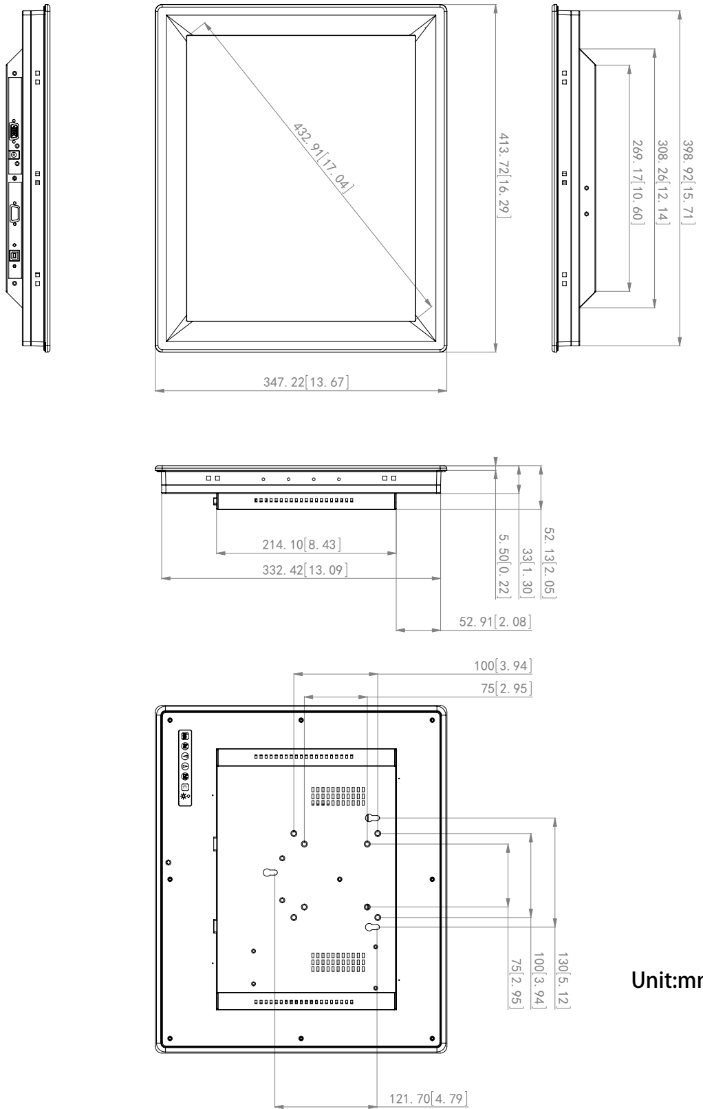
Figure 1.3 FPM-2170G Dimensions
