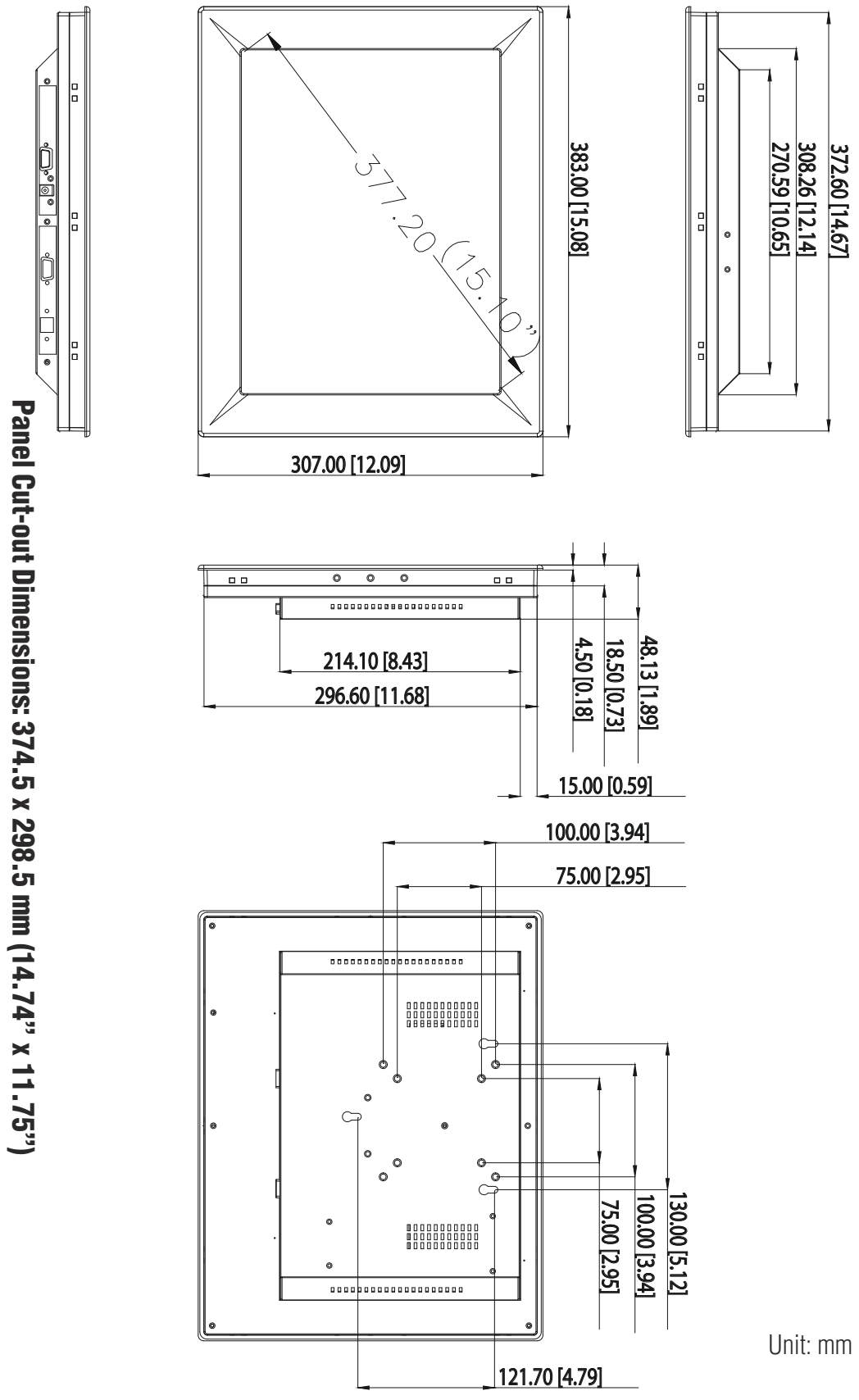
Figure 1.2 FPM-2150G Dimensions
