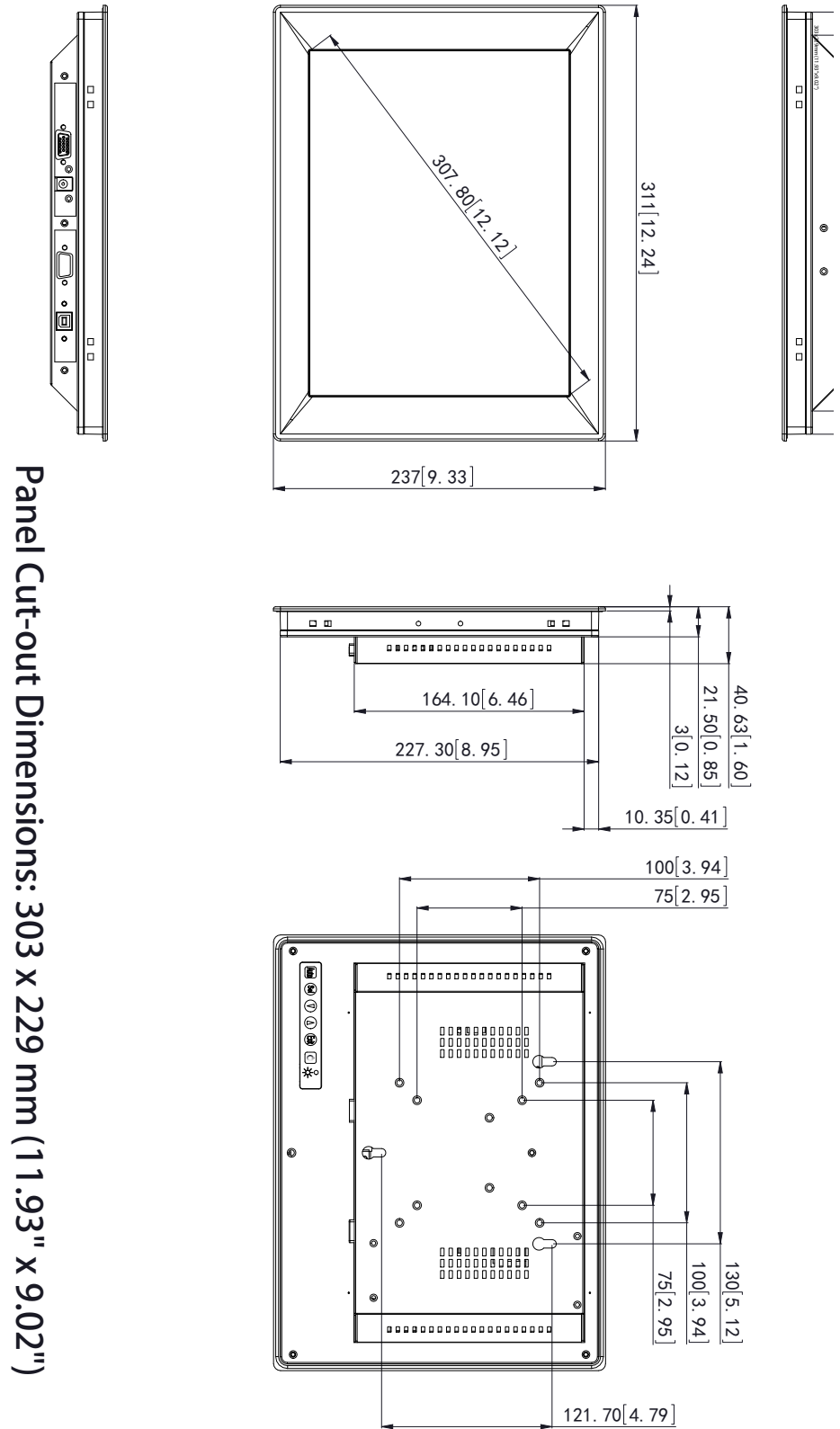
Figure 1.1 FPM-2120G Dimensions
