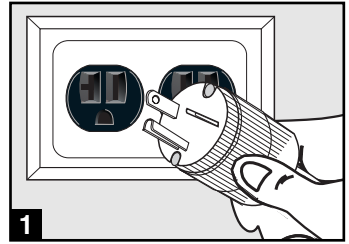
SMART2200RML2U plug (NEMA 5-20P) shown
