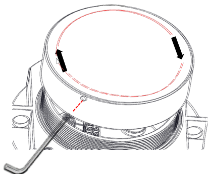
Figure 7. Installing D1005 cap
