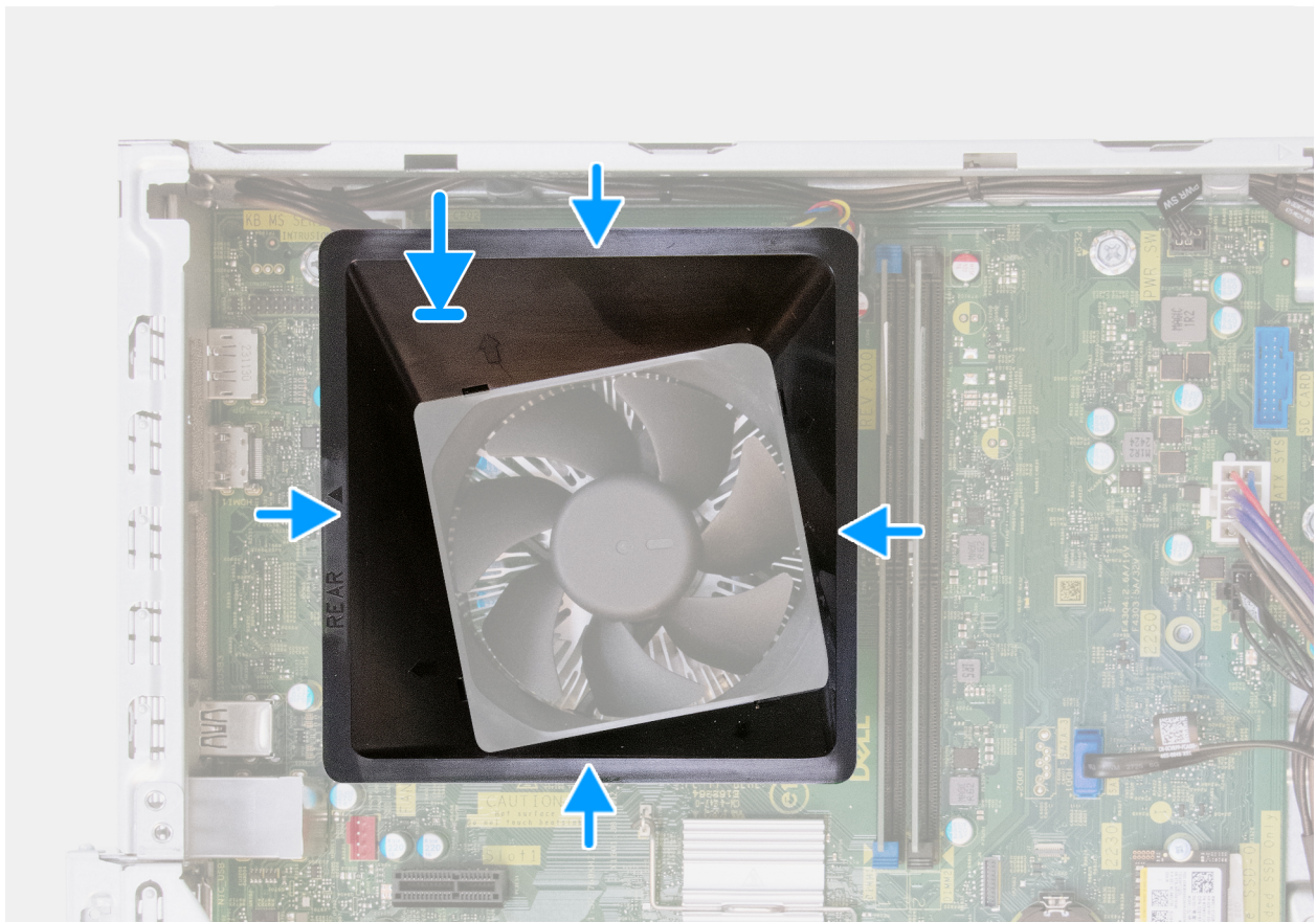
Figure 38. Installing the fan shroud
