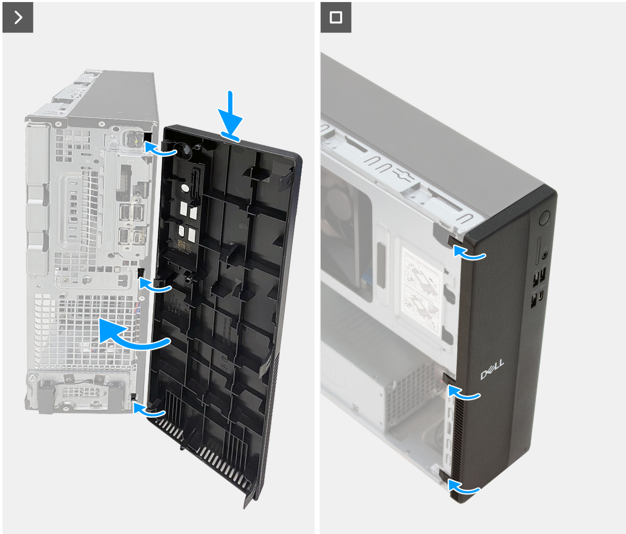
Figure 17. Installing the front cover
