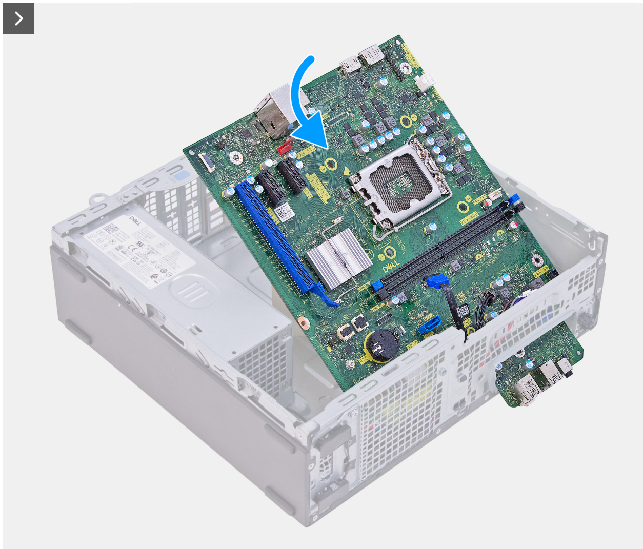
Figure 53. Installing the system board
