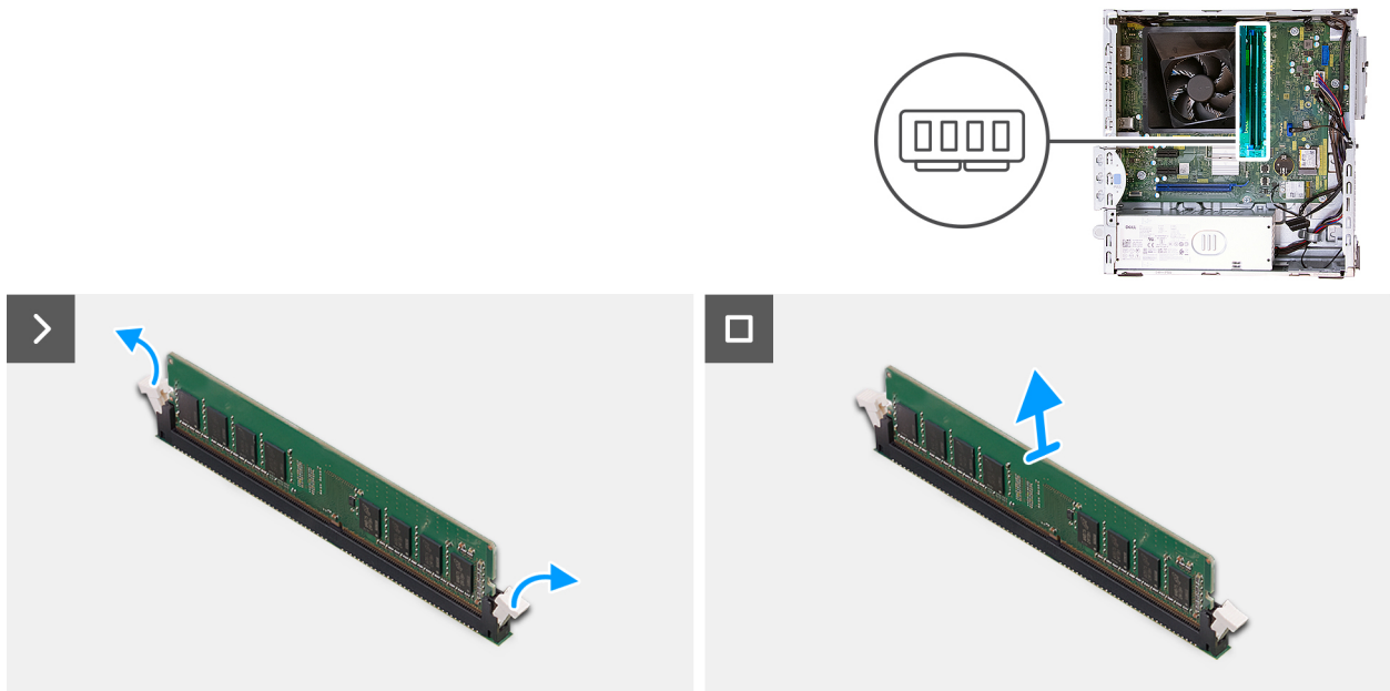
Figure 23. Removing a memory module
