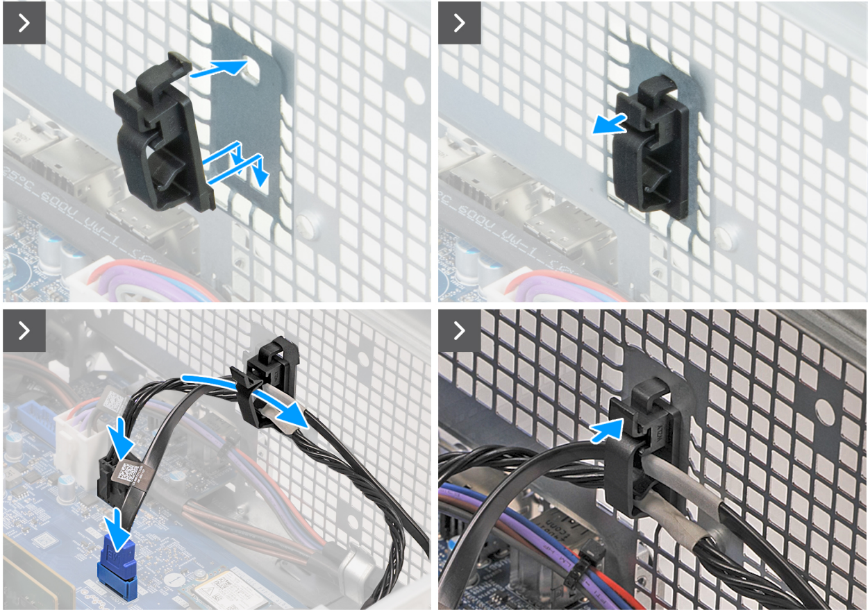
Figure 19. Installing the drive bay
