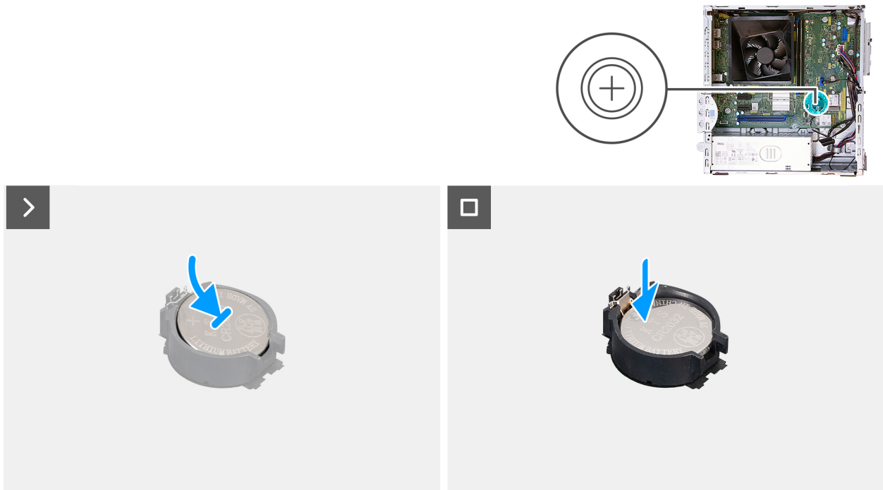
Figure 15. Installing the coin-cell battery
