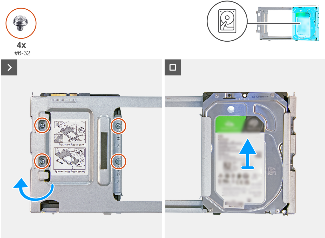
Figure 21. Removing the hard drive
