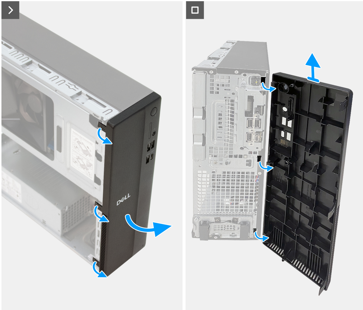
Figure 16. Removing the front cover
