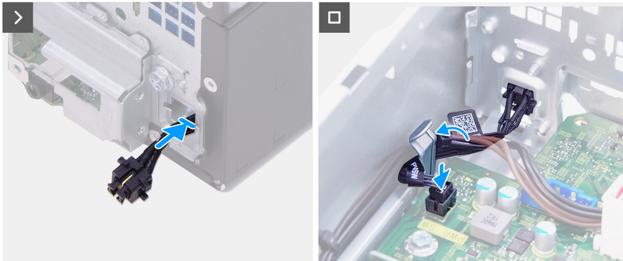
Figure 44. Installing the power button
