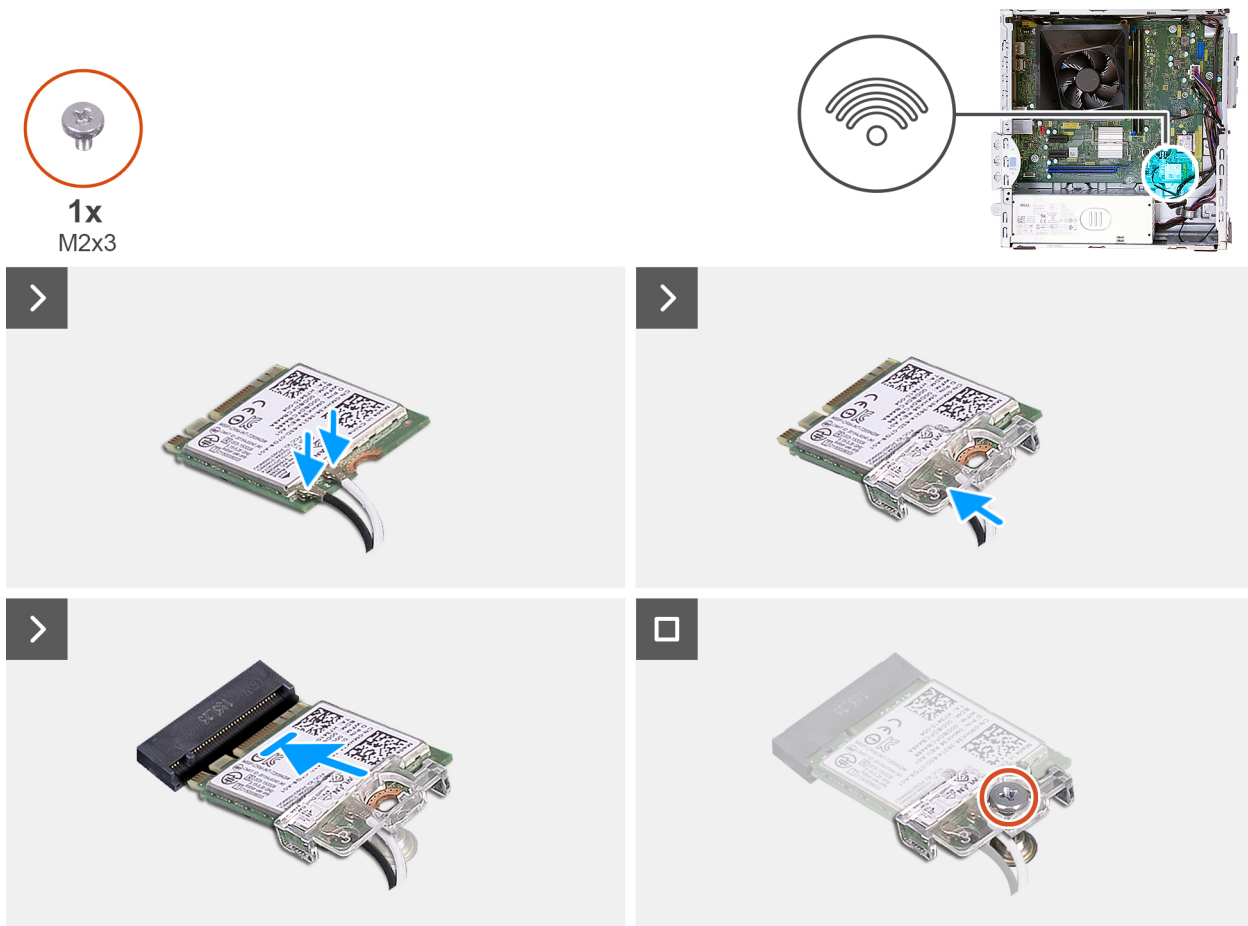
Figure 28. Installing the wireless card
