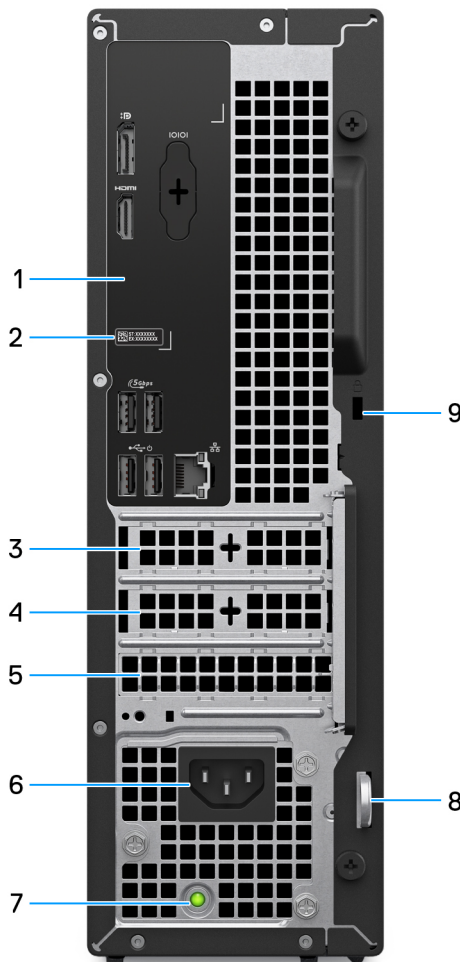
Figure 2. Back view of Dell Pro Slim Essential QVS1260
