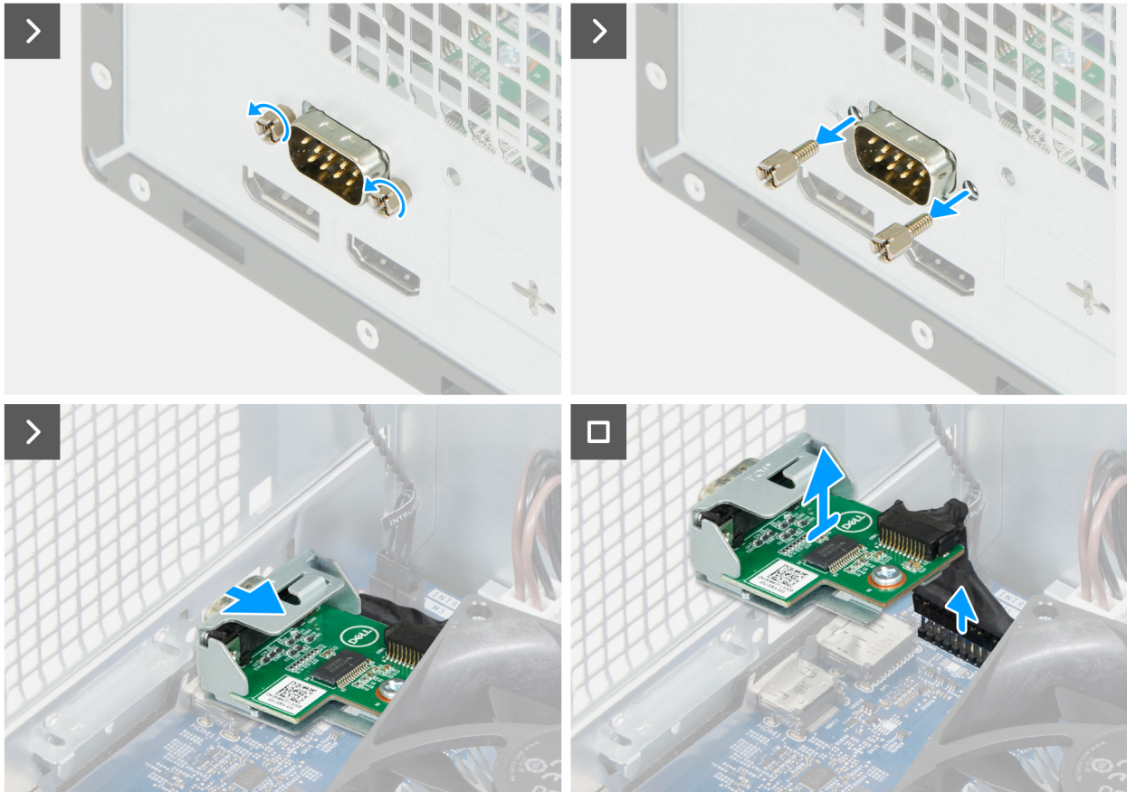
Figure 45. Removing the serial-port module
