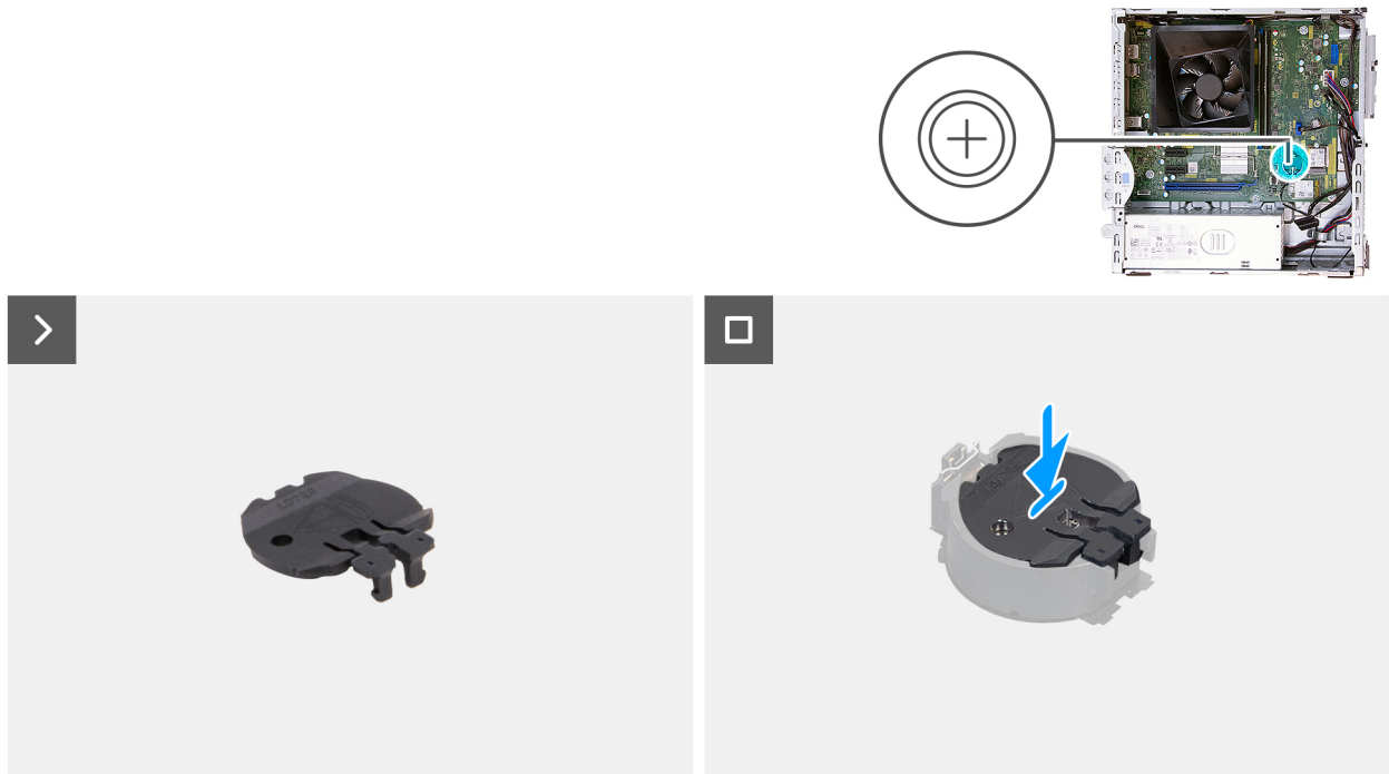
Figure 13. Installing the coin-cell battery cover
