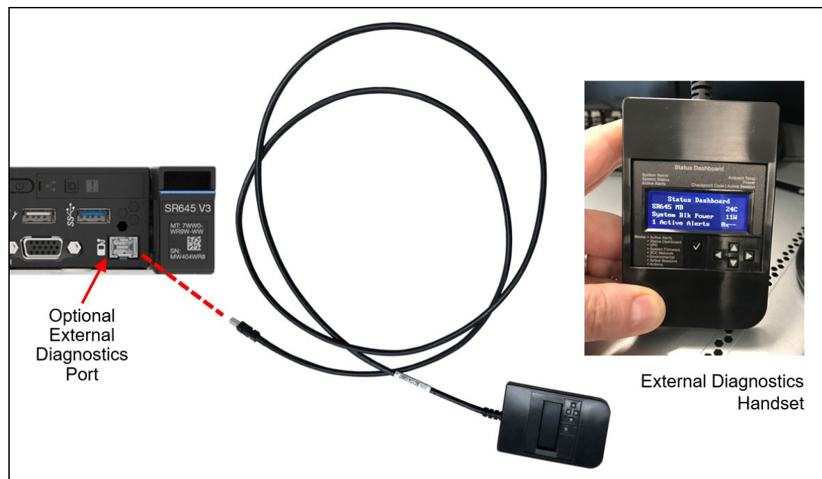
Figure 22. External Diagnostics Handset
