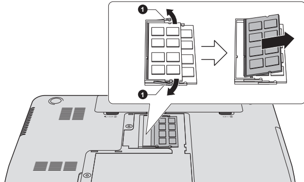
Figure 4-14 Removing the memory module(L830)
