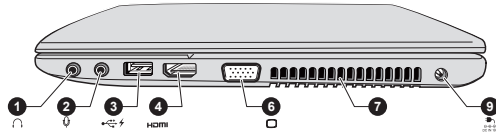
Figure 3-6 The right side of the computer(L840)
