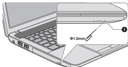
Figure 4-7 Manual release with the eject hole(L830)
