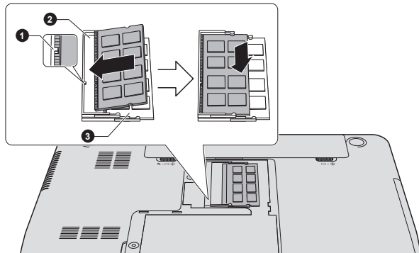
Figure 4-12 Seating the memory module(L830)
