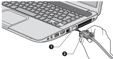
Figure 4-17 Connecting the monitor cable to the External RGB monitor port (L830)
