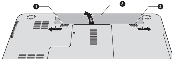
Figure 4-10 Releasing the battery pack -2(L830)
