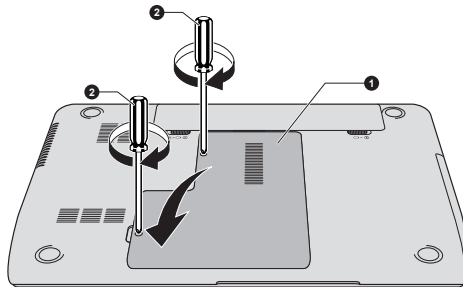
Figure 4-13 Seating the memory module cover(L830)
