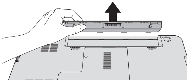
Figure 4-10 Releasing the battery pack -2(L830)
