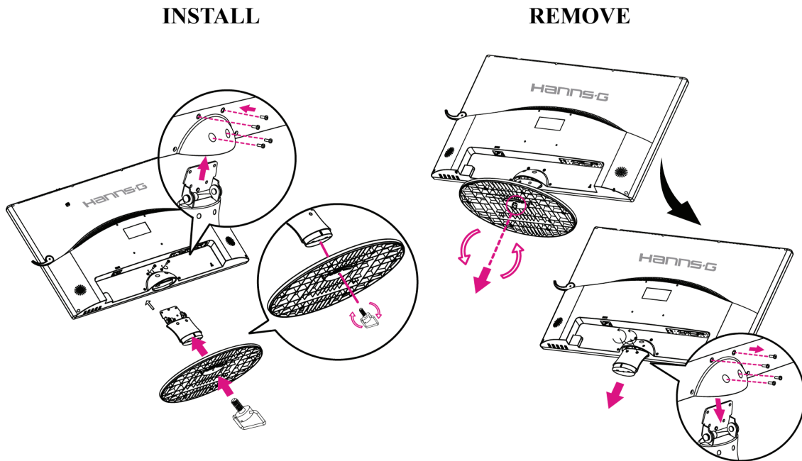
Figure.2. Installing and Removing the Base
