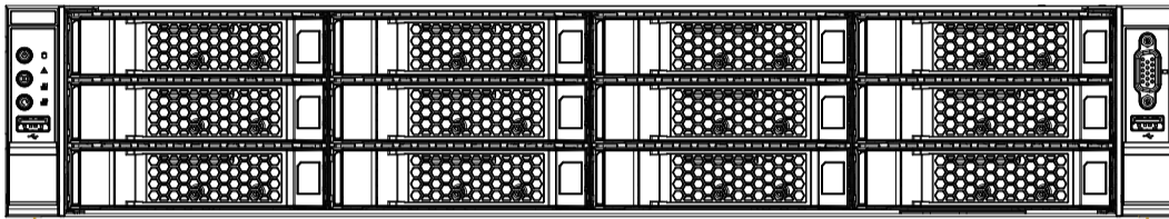
Front Panel Board Cable (Left, LED+USB2.0) (L=660/730mm) and Front Panel Board Cable (Right, VGA+USB3.0) (L=1100/1210mm)
