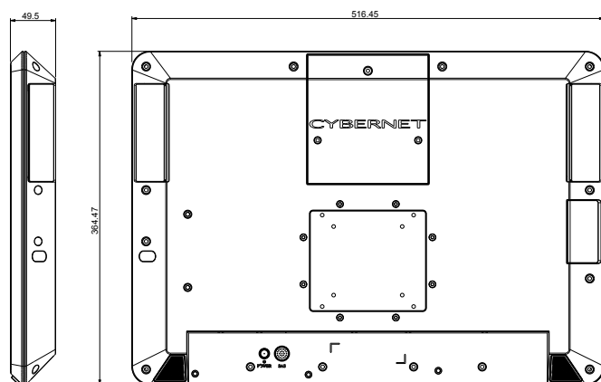
20" Medical Monitor
