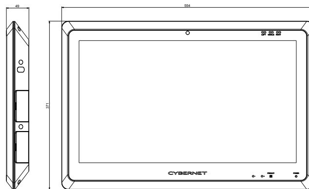
22" Medical Monitor
