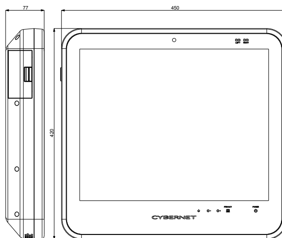
19" Medical Monitor
