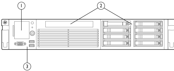
HP Integrity rx2800 i4 Server: Front View
