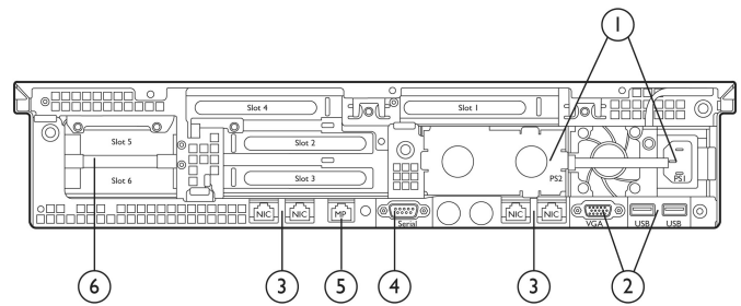
HP Integrity rx2800 i4 Server: Rear View
