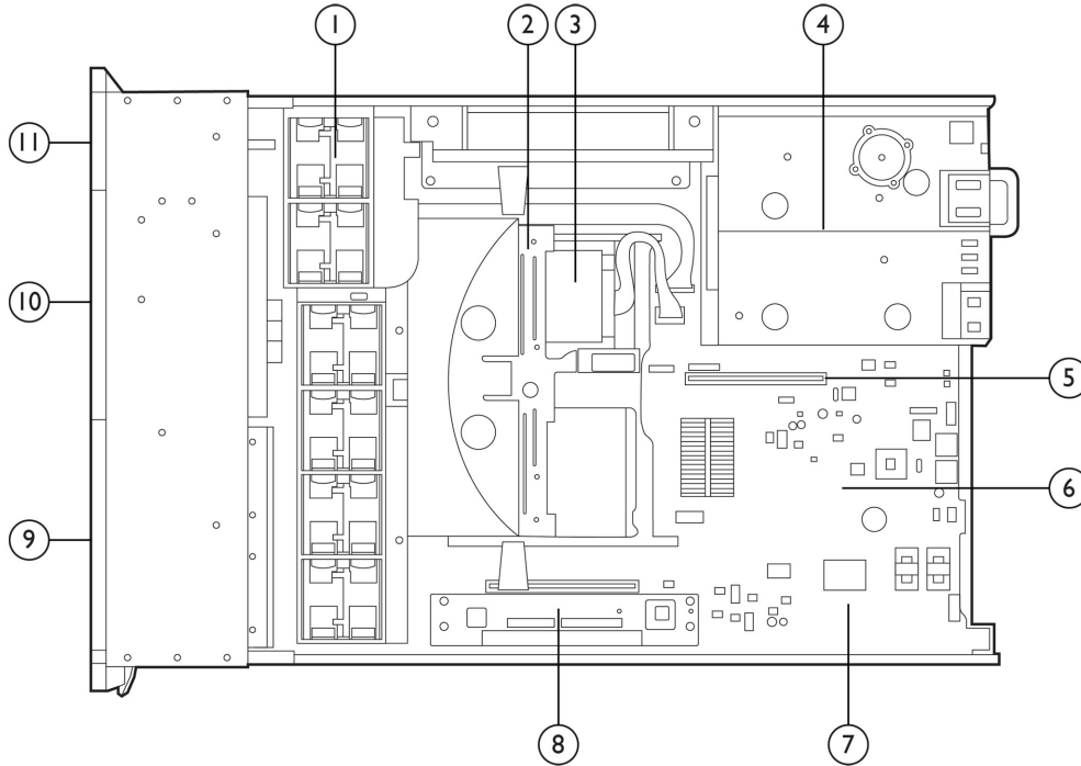
HP Integrity rx2800 i4 Server: Inside View
