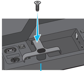
Holder-Cable
