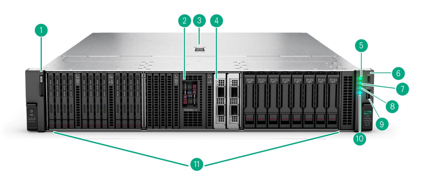
Front View - SFF/EDSFF CTO Server
