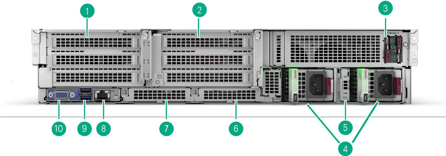
Rear View
