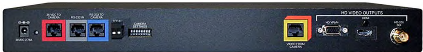
Image: Rear Panel CCU Connections and Controls (left to right)
