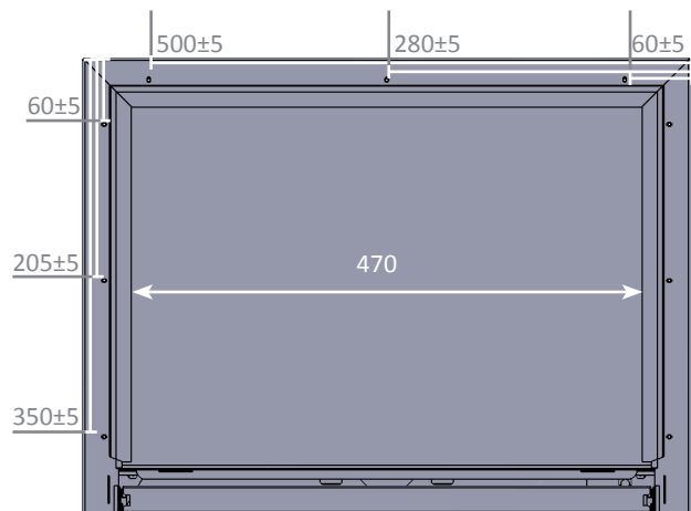
Dreamoc HD3 bottom - screw positions
