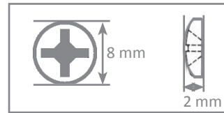
screw measurements
