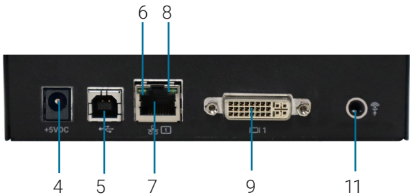
FIGURE 5-26. REAR VIEW OF THE EMERALD SE R2 DVI TRANSMITTER, DUAL-HEAD (EMD2000SE-T-R2)
