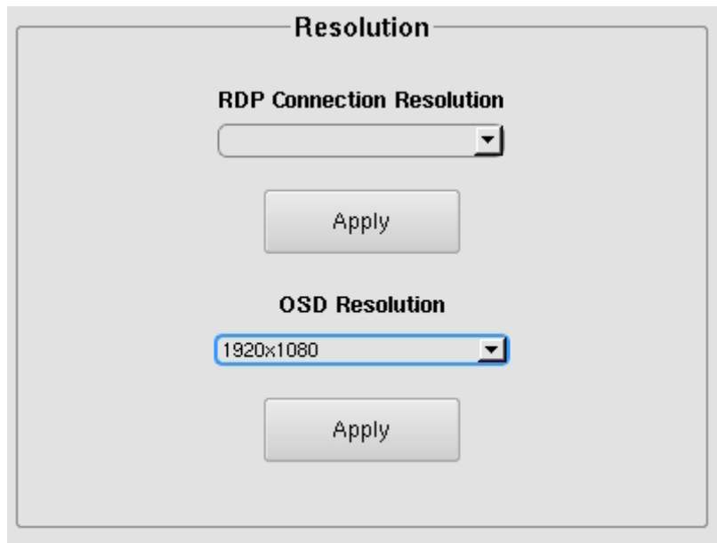
FIGURE 8-14. RESOLUTION SCREEN
