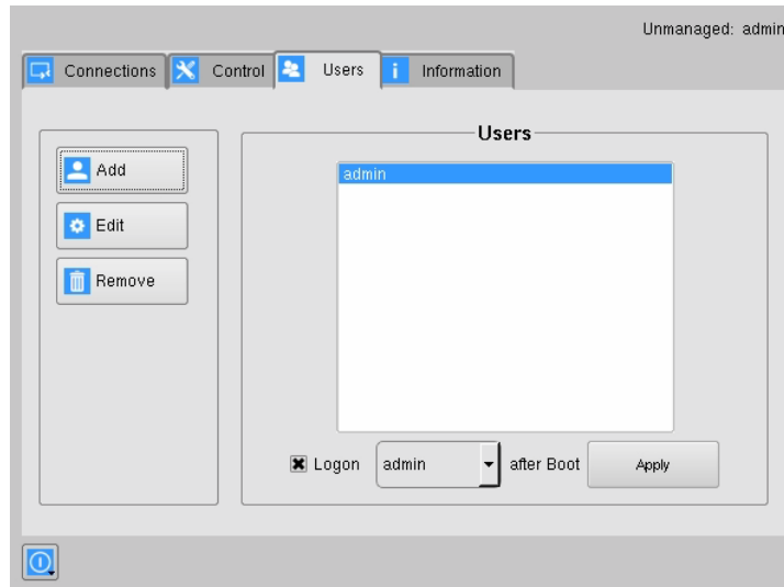
FIGURE 8-34. USER SCREENS
