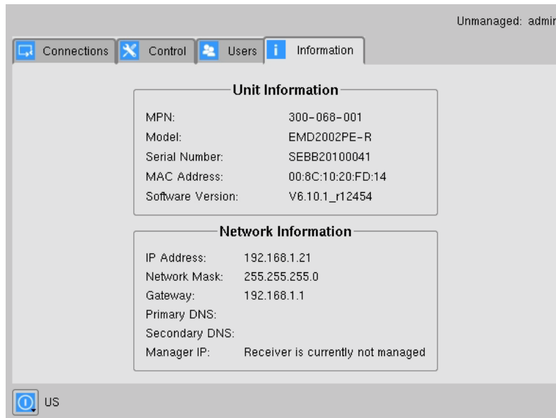
FIGURE 8-38. INFORMATION TAB
