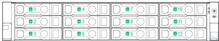
12 LFF + 2 rear SFF hot-plug drive model
