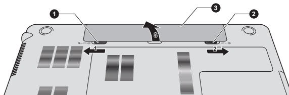
Figure 5-1 Releasing the battery pack -1
