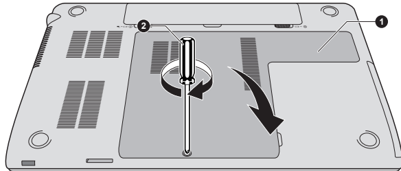
Figure 3-15 Seating the memory module cover
