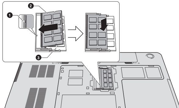
Figure 3-14 Seating the memory module
