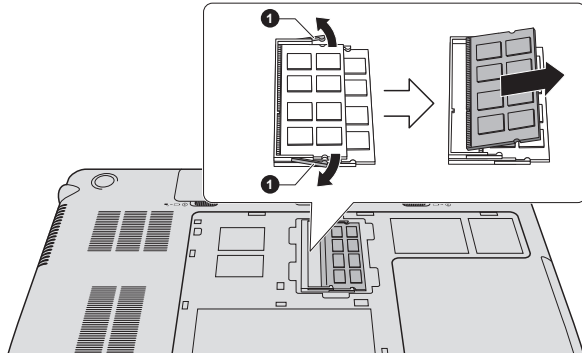
Figure 3-16 Removing the memory module
