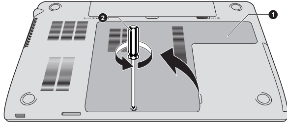
Figure 3-13 Removing the memory module cover
