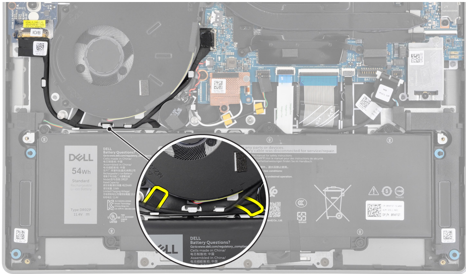
Figure 44. I/O-board cable routing
