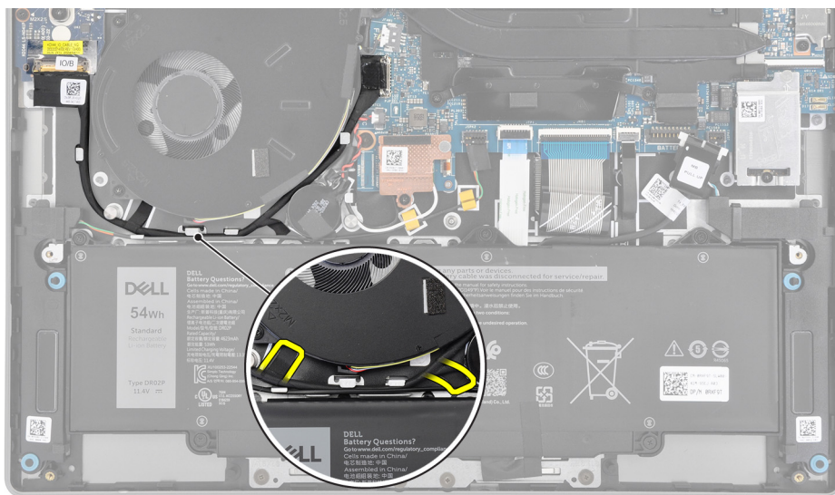
Figure 42. I/O-board cable routing
