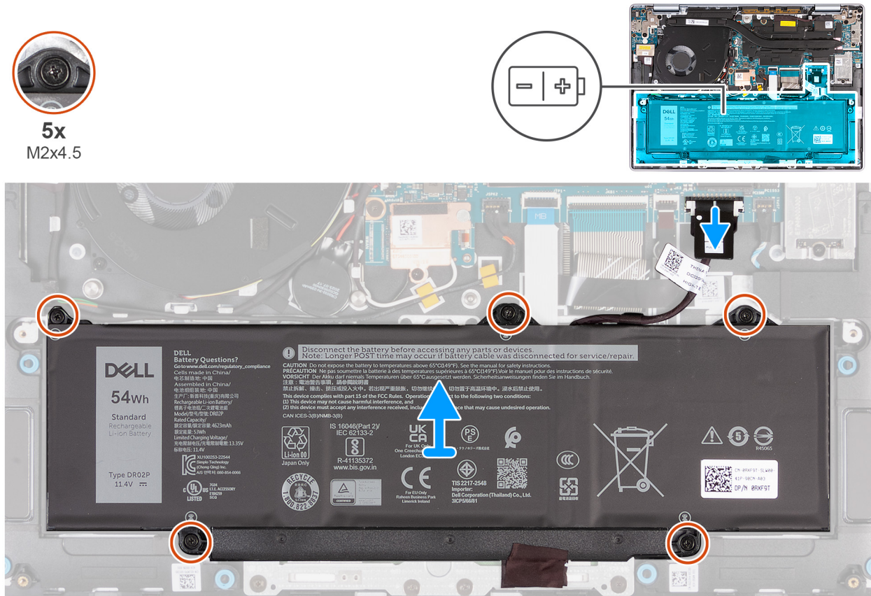
Figure 25. Removing the battery
