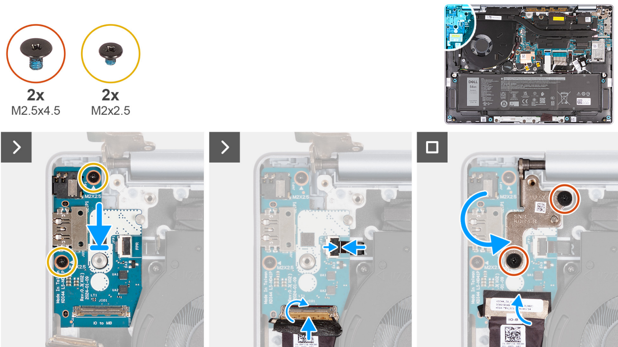
Figure 40. Installing the I/O board
