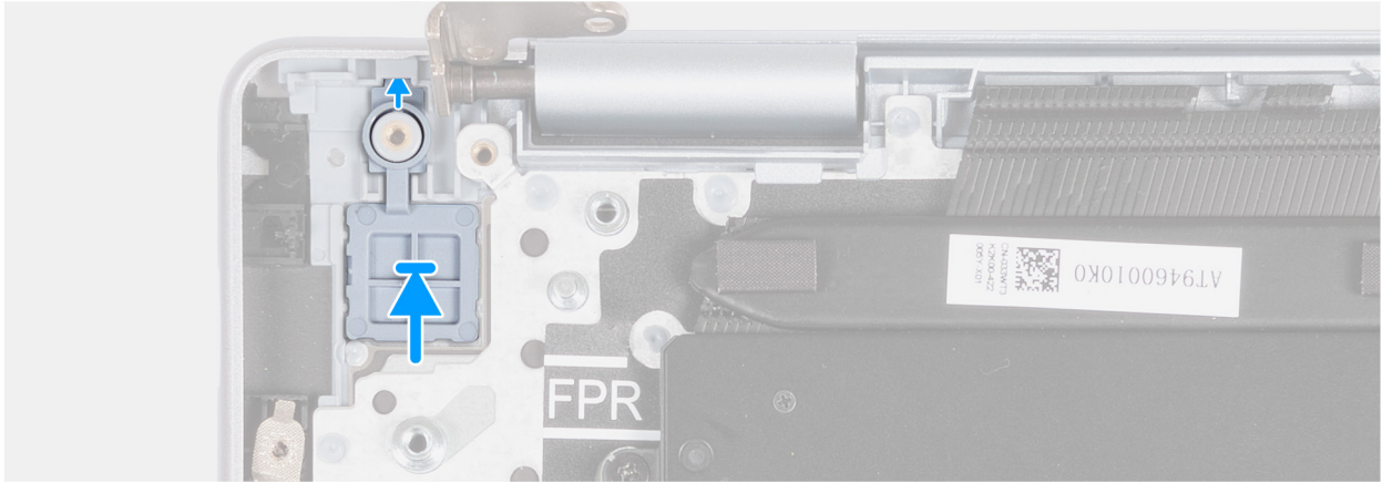
Figure 46. Installing the power button
