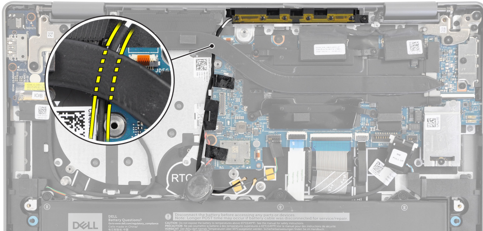
Figure 54. Installing antenna cables
