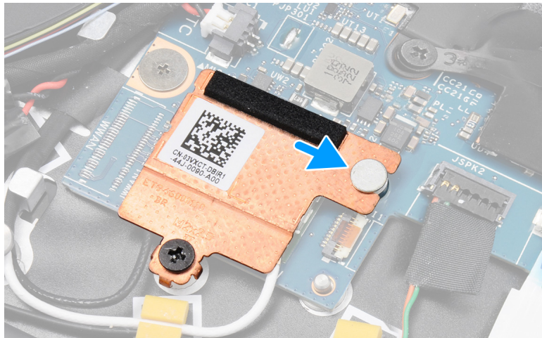
Figure 56. Installing wireless card thermal plate
