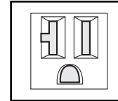
20 amp/120V NEMA 5-20R
