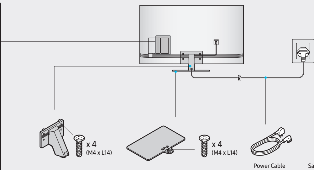
Power Cable
