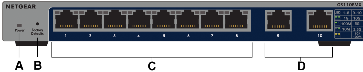
Figure 2. Front panel
