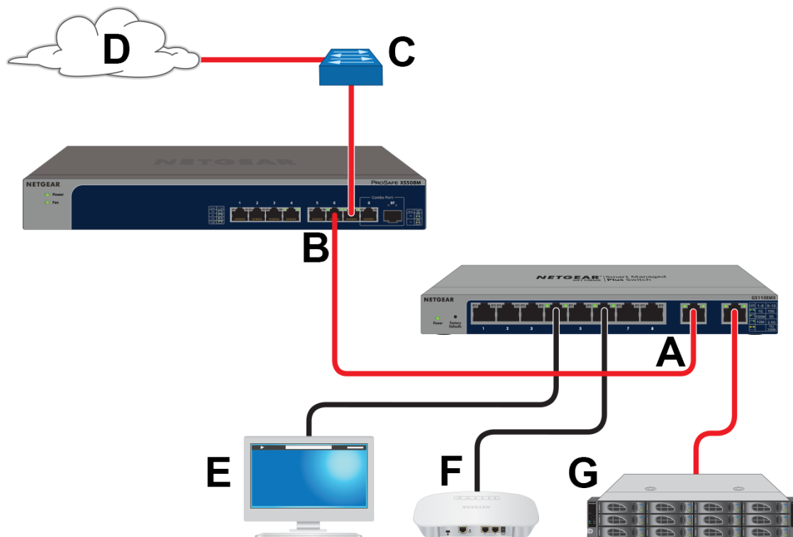
Figure 5. Sample connections
