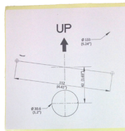
Drilling template
