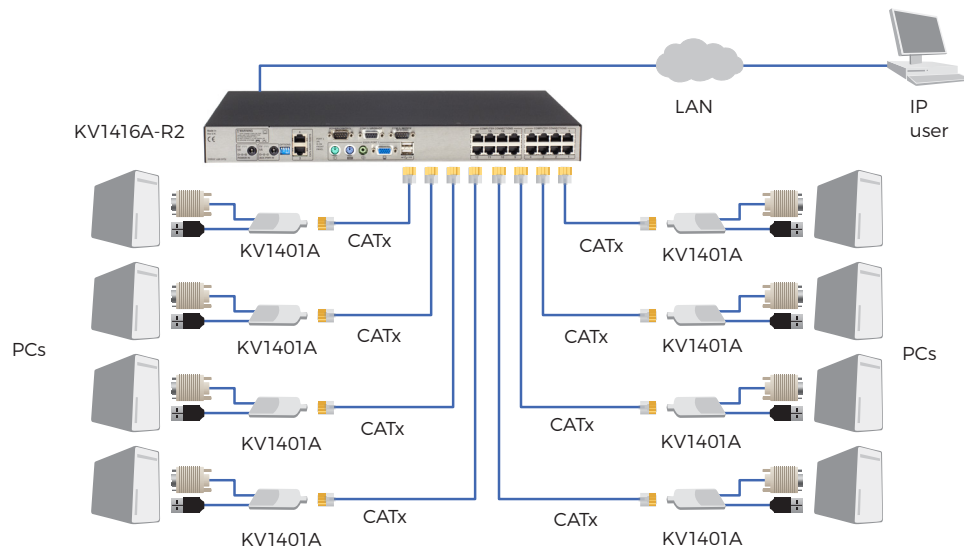
Figure 3-3. Application diagram #3.
