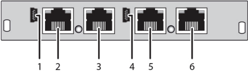
CATX DUAL REPEATER MODULE (ACX1M-2C2C)
