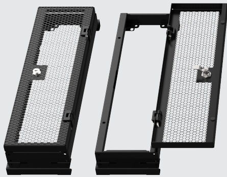
• 3U SECURITY COVER
