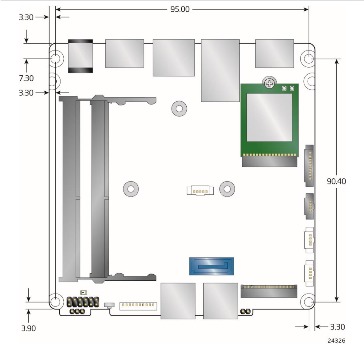
Figure 17. Board Dimensions
