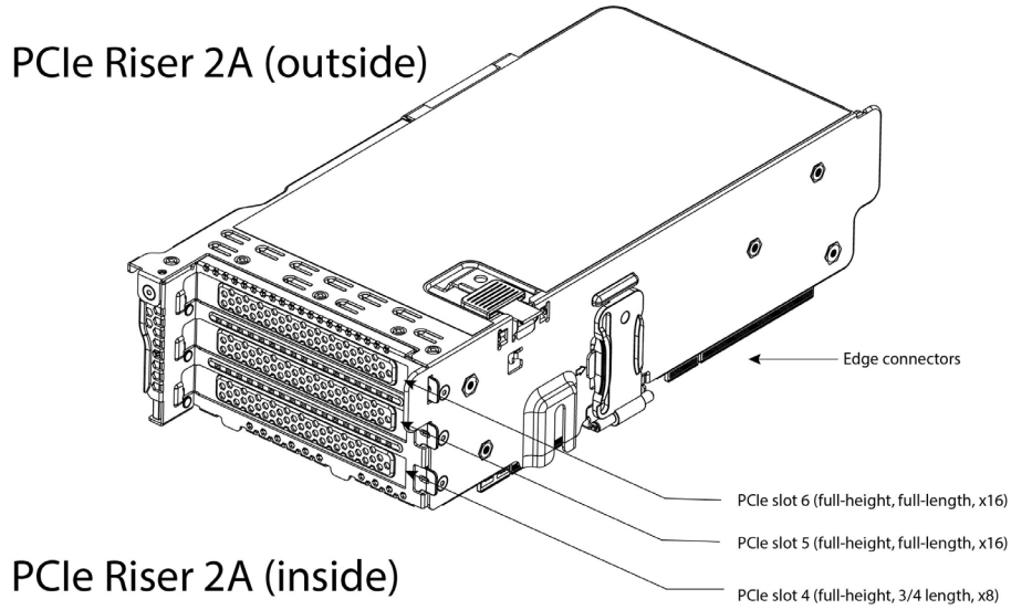
Figure 11 Riser Card 2A
