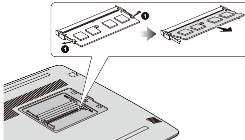
Figure 4-6 Removing the memory module
