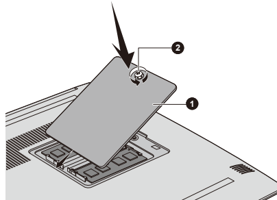
Figure 4-5 Seating the memory module cover
