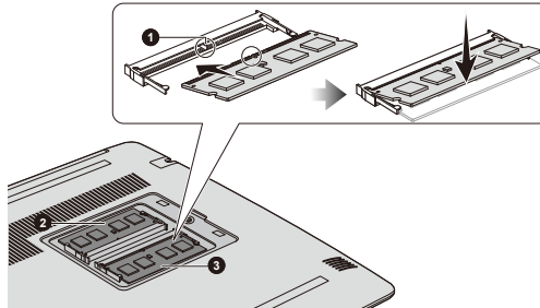
Figure 4-4 Seating the memory module
