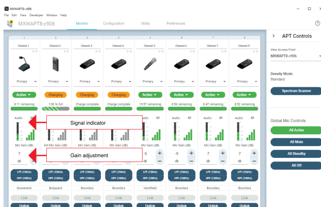
Monitor Tab
